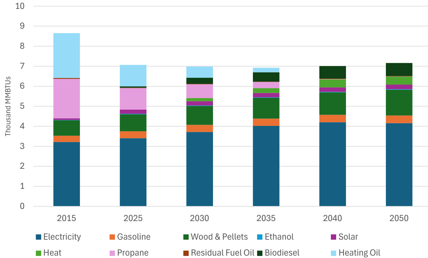
Sandgate Commercial Energy Demand
