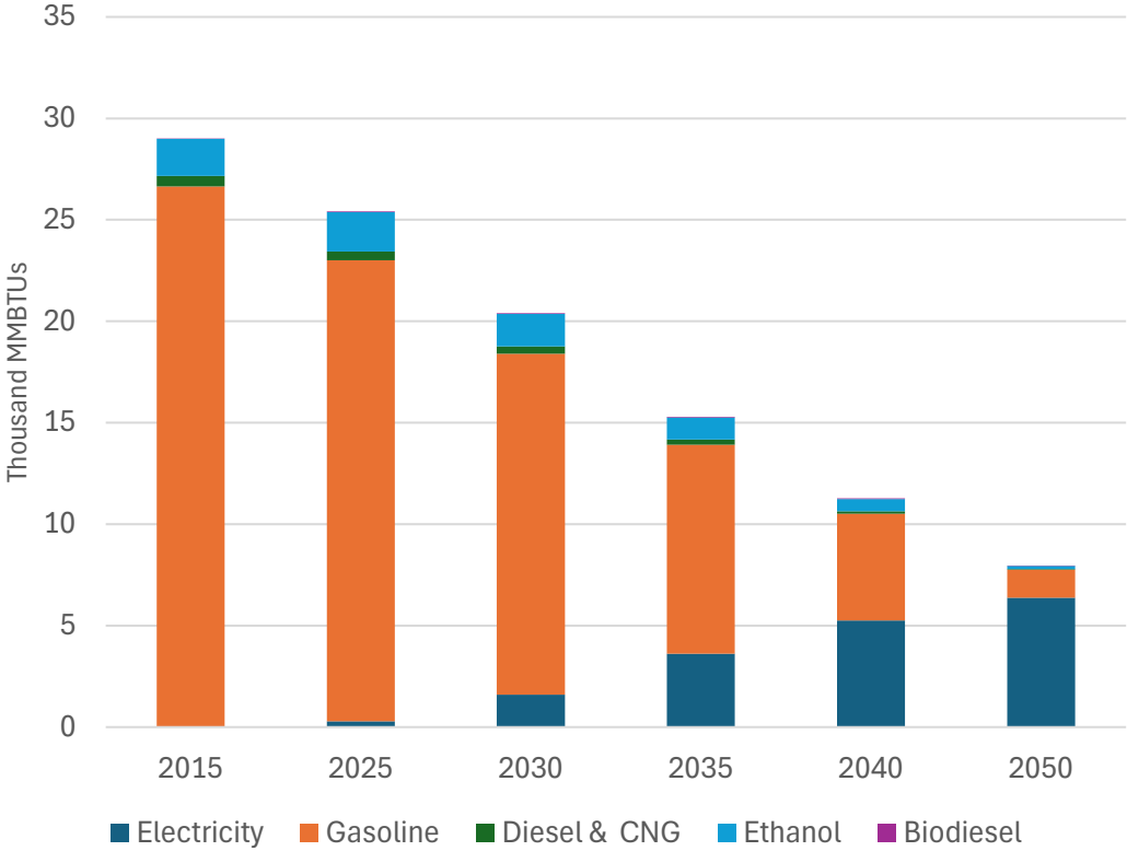
Sandgate Light Truck Energy Demand
