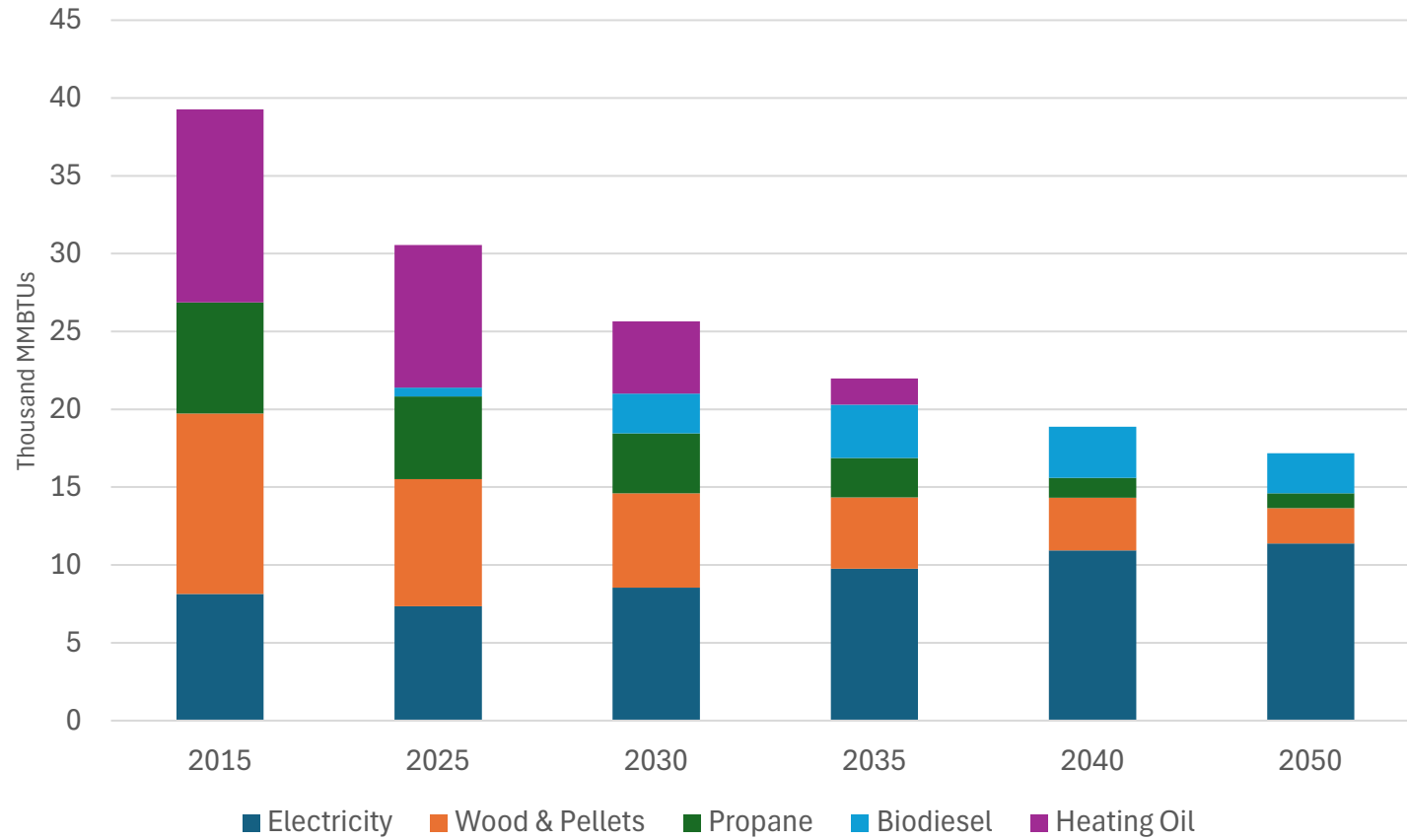
Sandgate Residential Energy Demand
