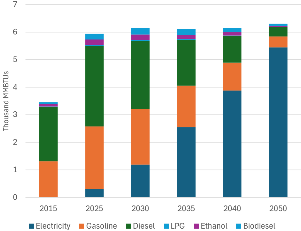
Sandgate Medium Truck Energy Demand
