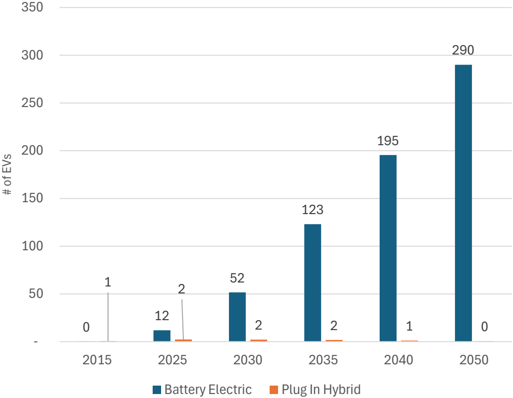
Sandgate EV and PHEV Targets
