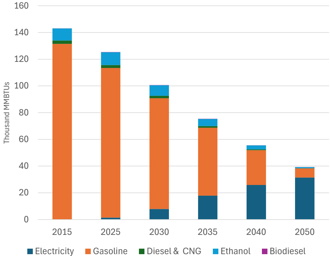
Pownal Light Truck Energy Demand
