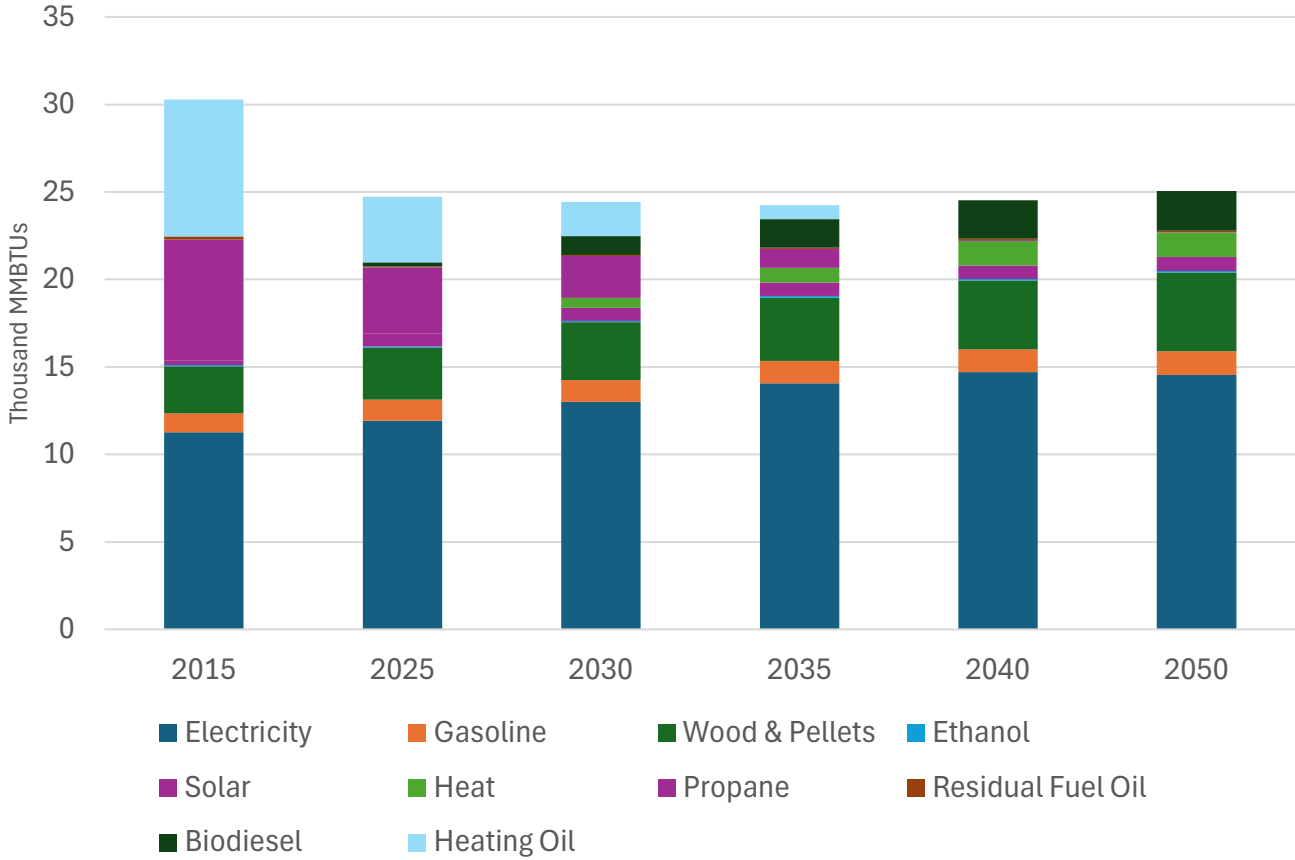
Pownal Commercial Energy Demand
