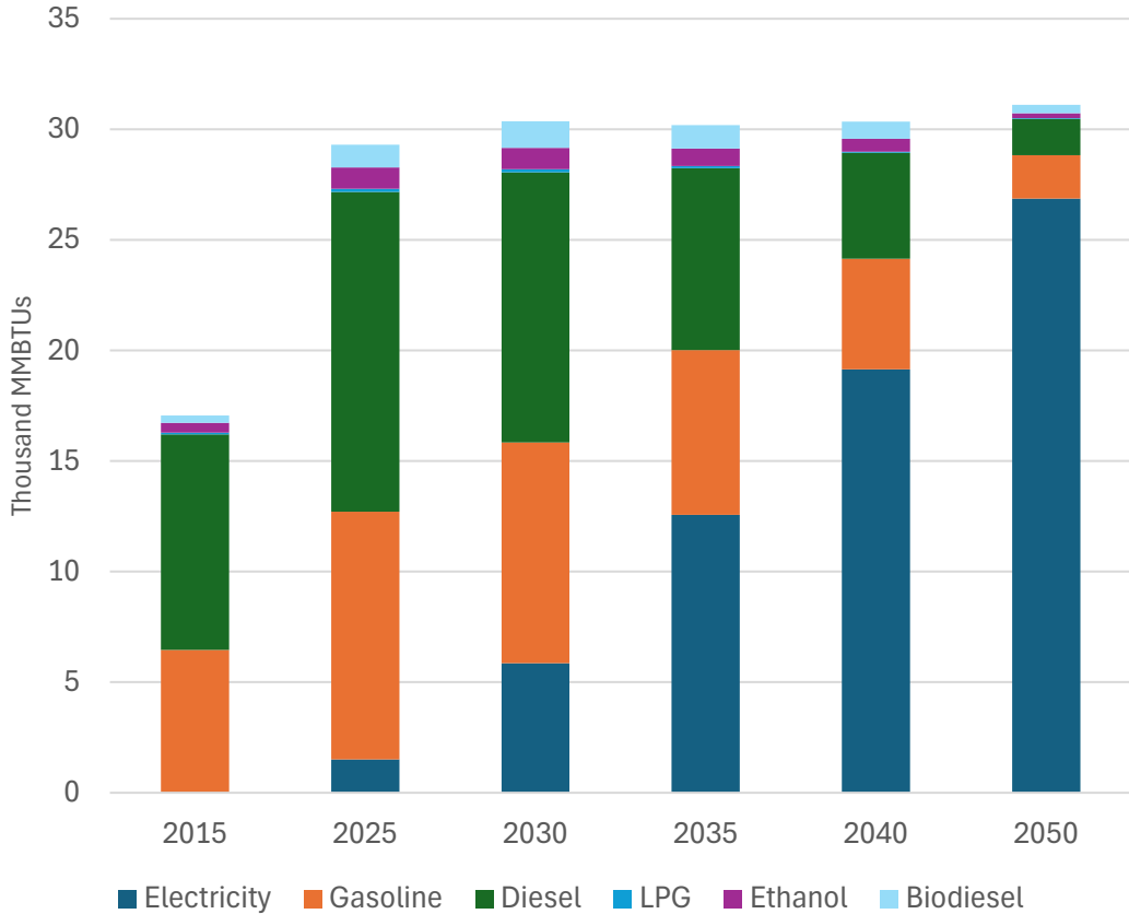
Pownal Medium Duty Truck Energy Demand
